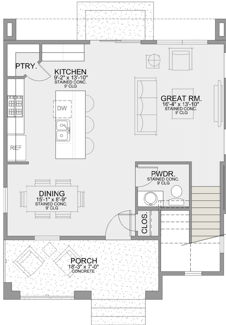
FIRST FLOOR PLAN LIVING AREA: 653 SF
