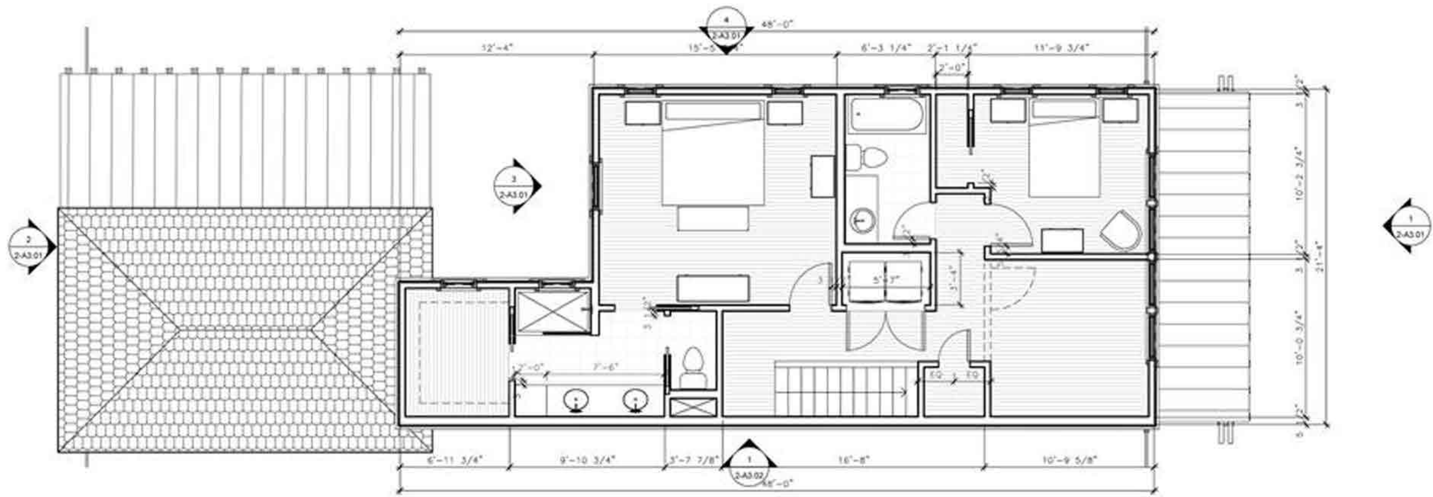
2 UNIT 2 - 02 FLOOR 1/4" = 1'-0"
